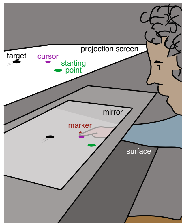
Fig. 1 Schematic representation of the set-up. A target, cursor, and starting point were projected from above onto a back-projection screen. The participant looked at the screen from below by looking into a mirror that blocked his or her view of the hand. The distance between the projection screen and the mirror was equal to that between the mirror and the surface across which the finger moved, so the items on the screen appeared to be on that surface. The participant's task was to slide his or her unseen finger across the surface, such that the cursor passed through the moving target. The cursor followed the position of the marker attached to the fingernail. The starting point and target were never present at the same time
