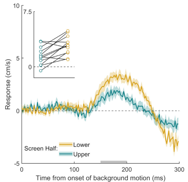
Figure 6. Time course of the response to background motion in Experiment 5. The gold curve shows the response to background motion in the lower half of the display, and the turquoise curve shows the response to background motion in the upper half of the display. Further figure details are the same as Figure 2 .
